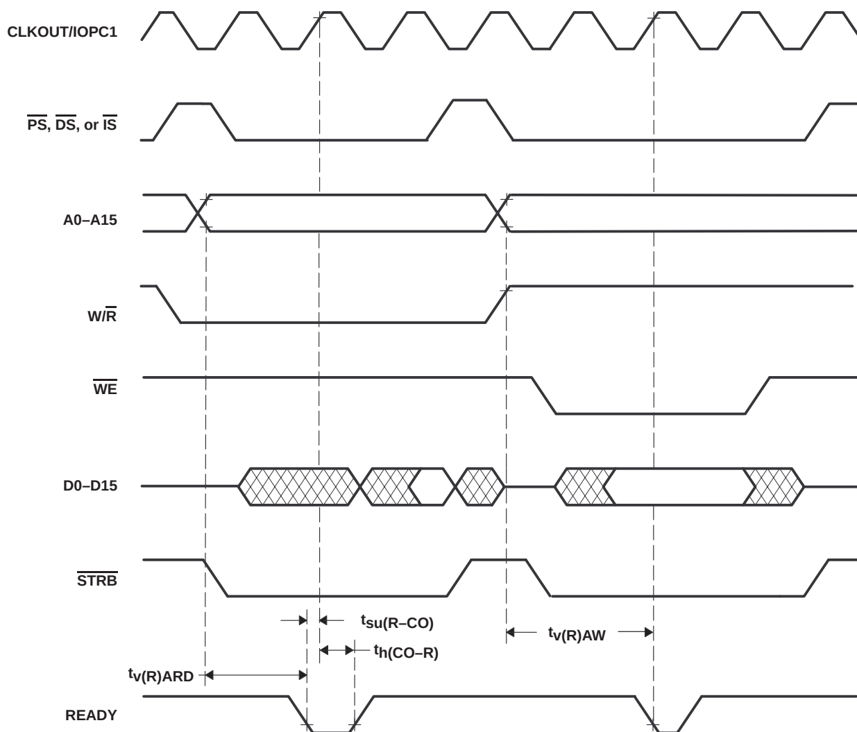
Figure 30. READY Timings
