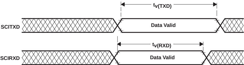
Figure 42. SCI Timings
