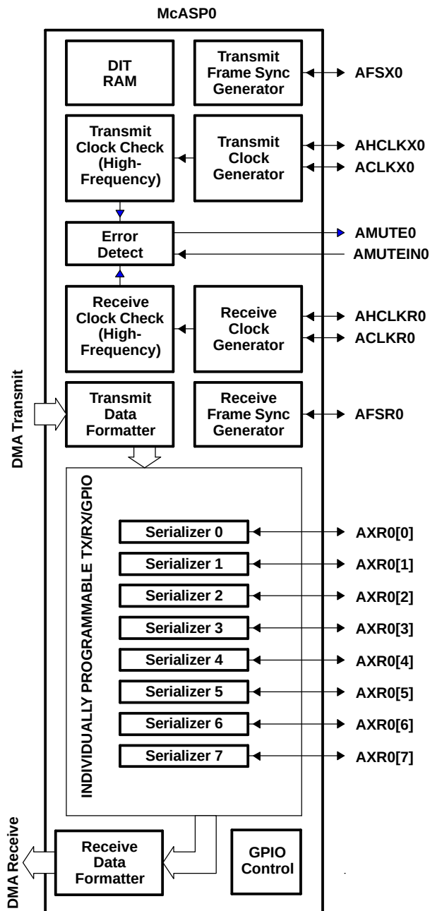
Figure 5-32. McASP0 Configuration
