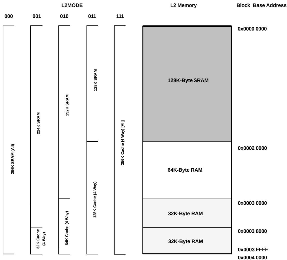
Figure 2-2. TMS320DM642 L2 Architecture Memory Configuration
