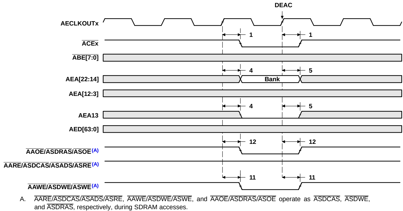
Figure 5-26. SDRAM DEAC Command for EMIFA
