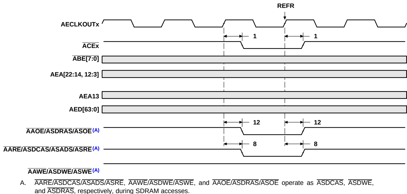
Figure 5-27. SDRAM REFR Command for EMIFA
