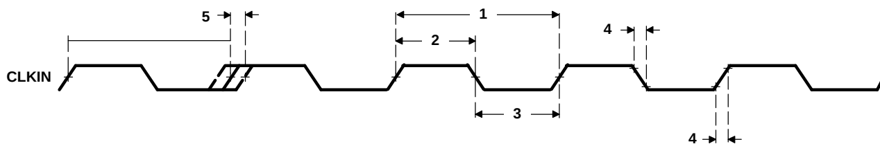
Figure 5-11. CLKIN Timing
