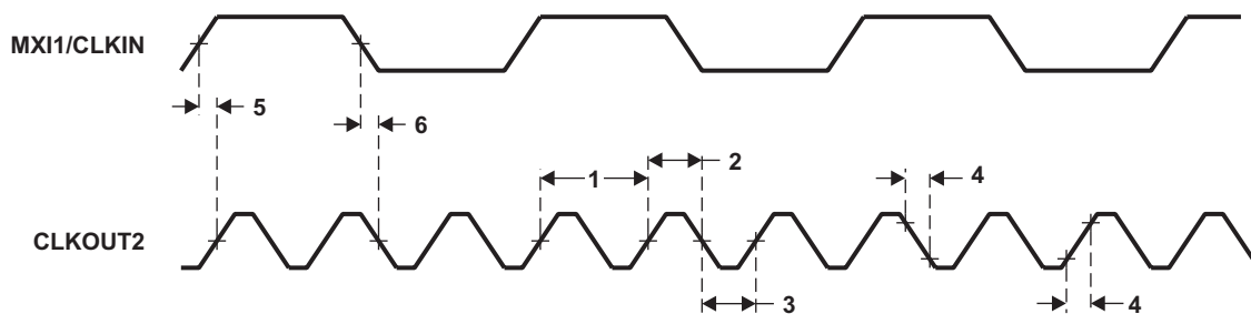
Figure 6-8. CLKOUT2 Timing
