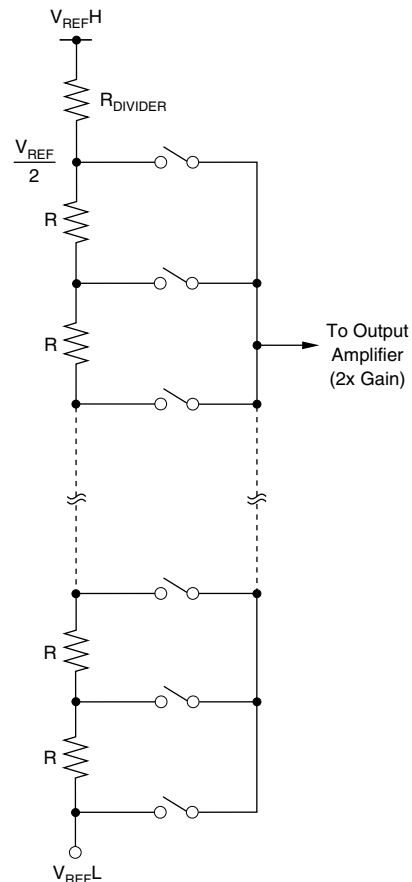
Figure 48. Resistor String
