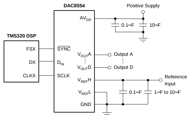
Figure 55. DAC8554 to TMS320 DSP
