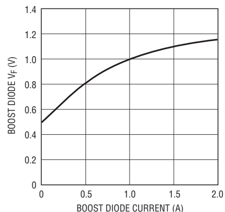
Boost Diode
