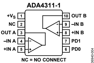
Figure 4. Pin Configuration
