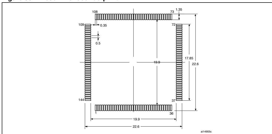
Figure 80. Recommended footprint
