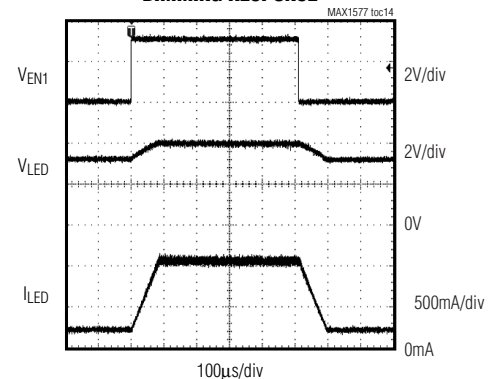
DIMMING RESPONSE
