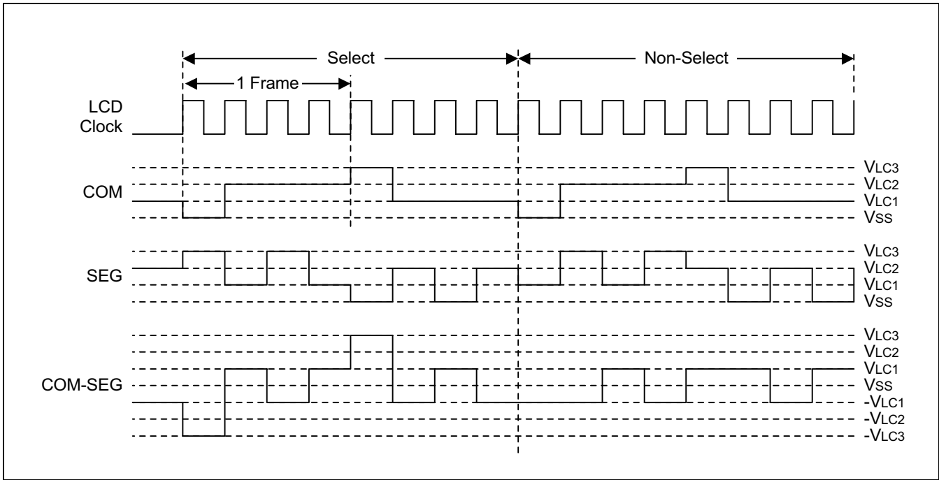
Figure 14-7. Select/No-Select Bias Signals in 1/4 Duty, 1/3 Bias Display Mode
