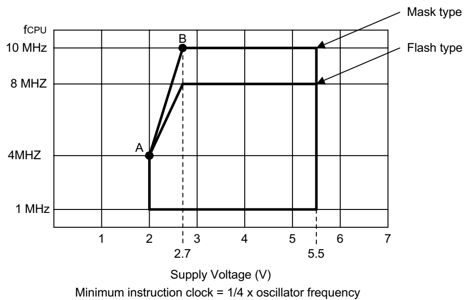
Figure 21-5. Operating Voltage Range
