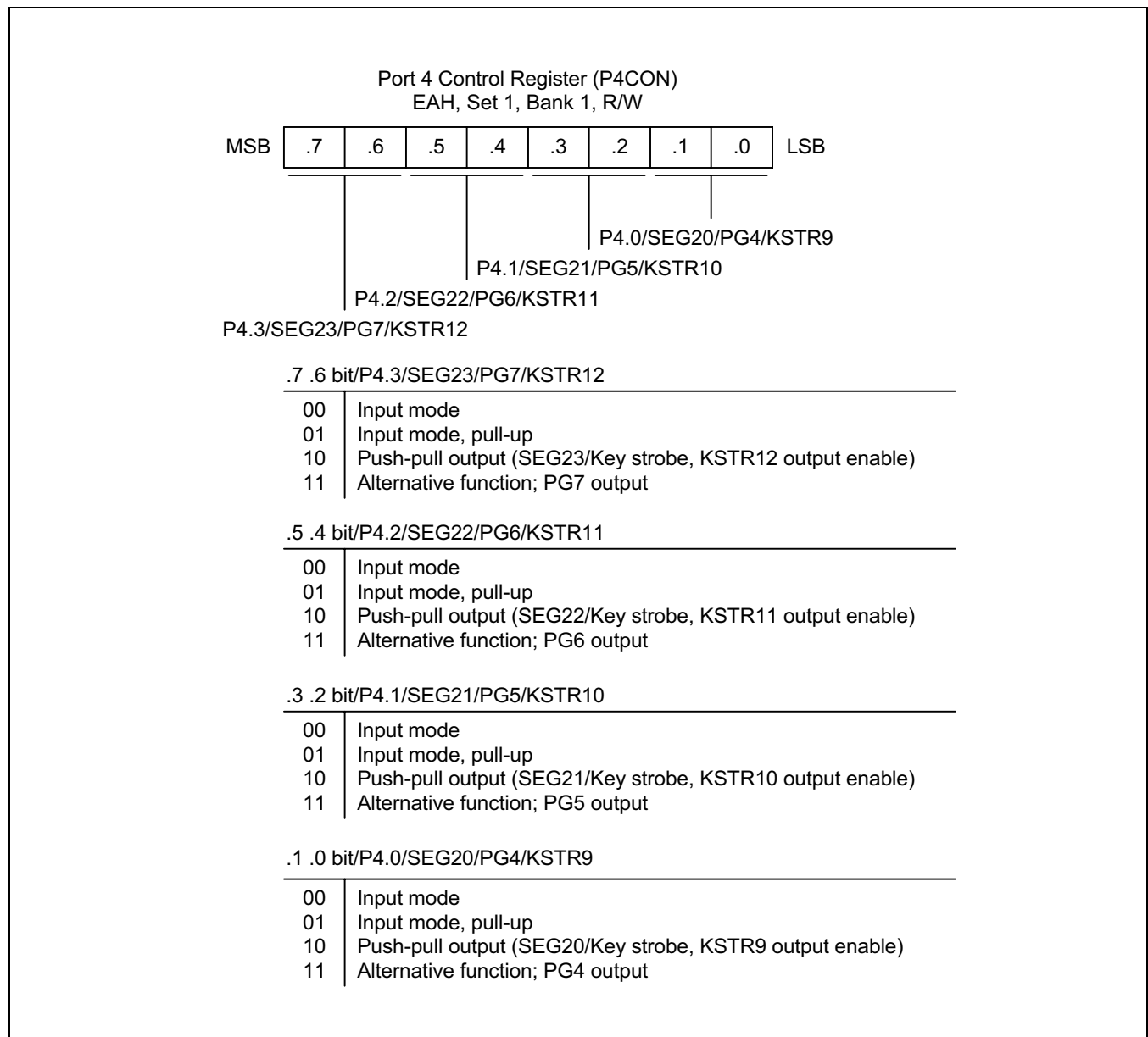
Figure 9-13. Port 4 Control Register (P4CON)
