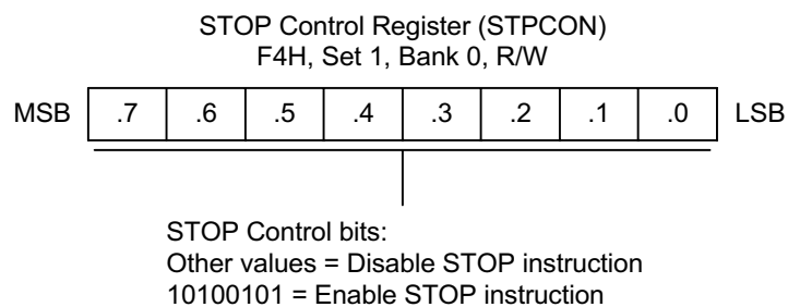
Figure 7-6. STOP Control Register (STPCON)
