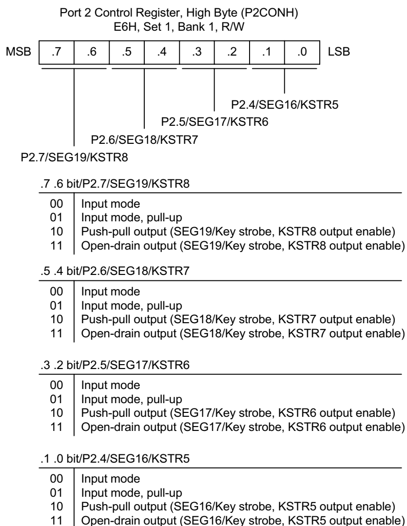
Figure 9-8. Port 2 High-Byte Control Register (P2CONH)
