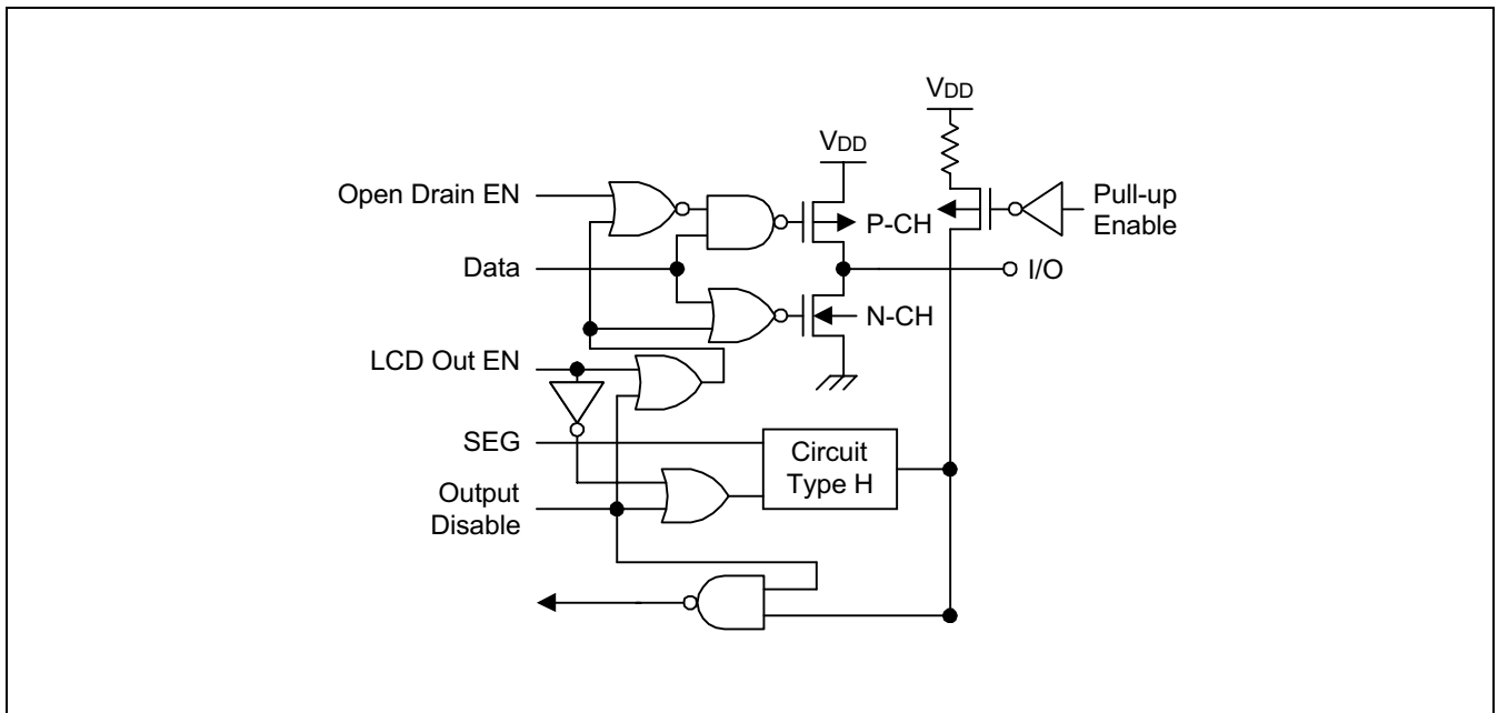
Figure 1-14. Pin Circuit Type H-14 (P2, P4)
