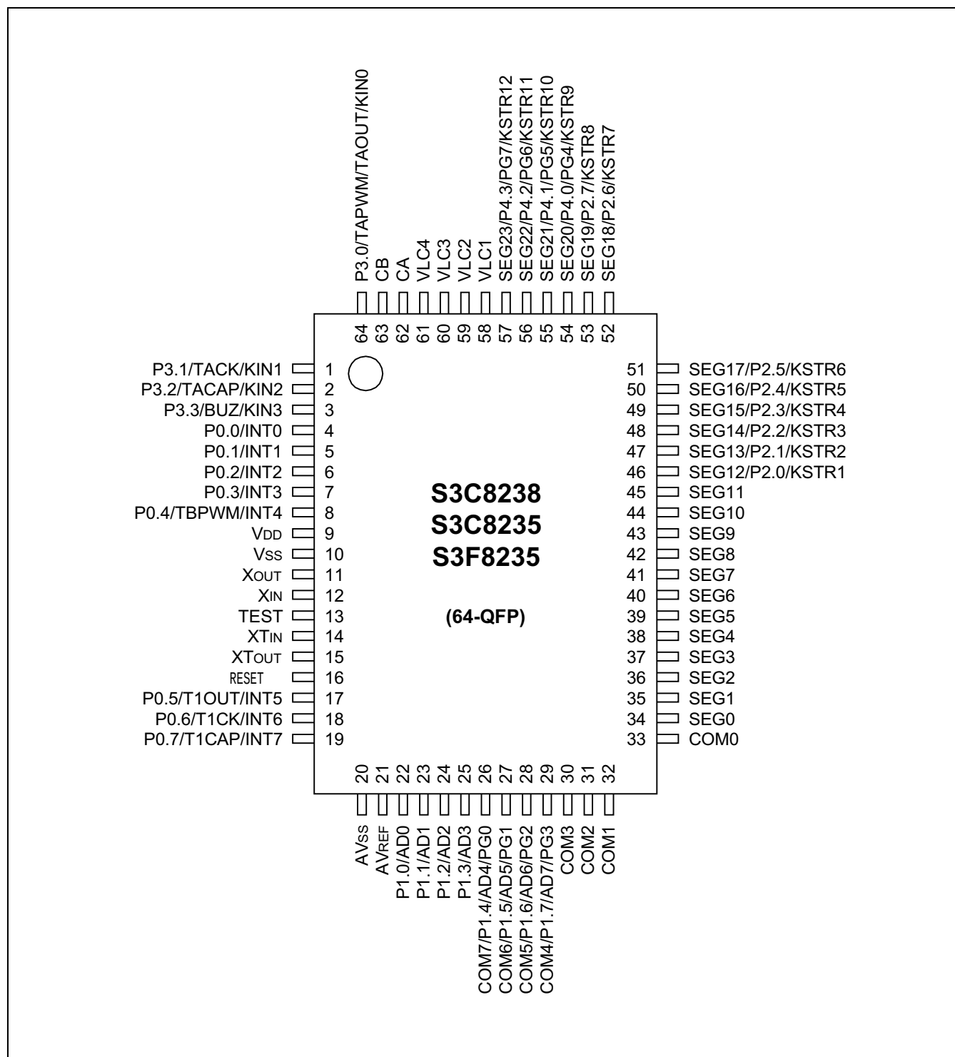
Figure 1-3. S3C8238/C8235/F8235 Pin Assignment (64-QFP)
