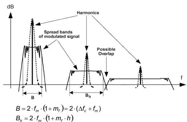
Figure 50. Spread Bands of Harmonics in Modulated Square Signals
