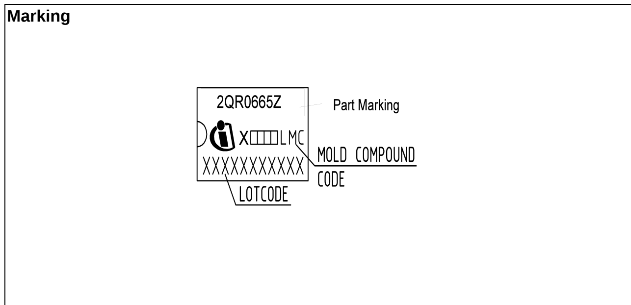
Figure 15 Marking for ICE2QR0665Z
