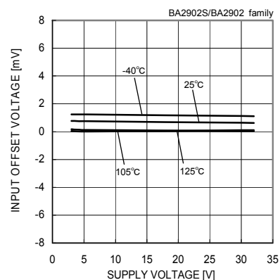
Fig. 84 Input Offset Voltage - Supply Voltage (Vcm=0[V], VOUT=1.4[V])
