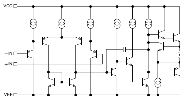
BA10358/BA10324A/BA2904S/BA2904/ BA2902S/BA2902/BA2904H simplified schematic
