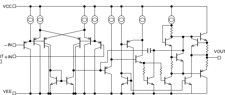
BA3404 simplified schematic
