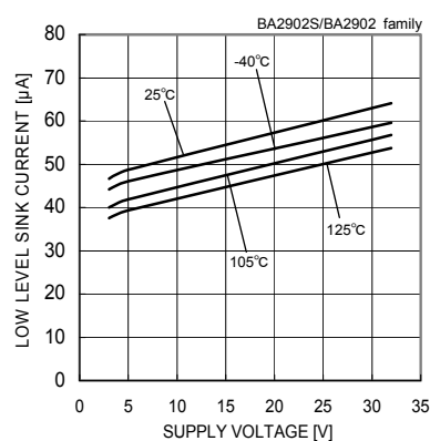
Fig. 82 Low Level Sink Current - Supply Voltage (VOUT=0.2[V])
