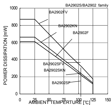
Fig. 73 Derating Curve
