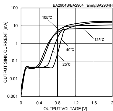
Fig. 56 Output Sink Current - Output Voltage (VCC=5[V])
