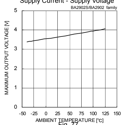
Fig. 77 Maximum Output Voltage - Ambient Temperature (VCC=5[V], RL=2[kΩ])
