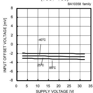
Fig. 12 Input Offset Voltage - Supply Voltage (Vcm=0[V], VOUT=1.4[V])
