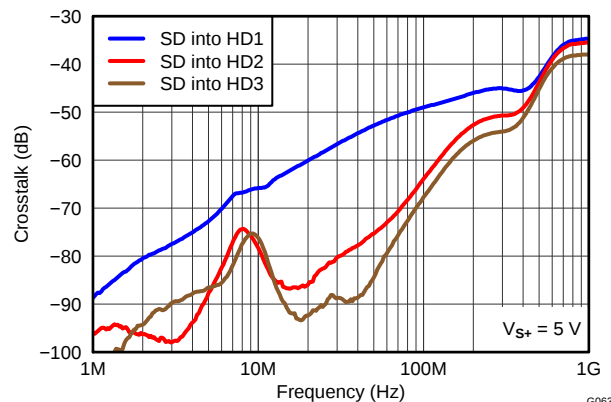
Figure 75. SD-TO-HD BYPASS CROSSTALK vs FREQUENCY
