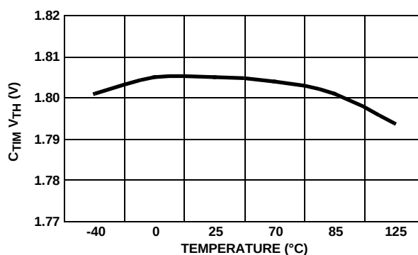
FIGURE 5. C_{TIM} OC VOLTAGE THRESHOLD
