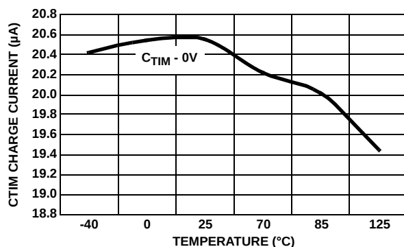
FIGURE 4. C_{TIM} CURRENT SOURCE
