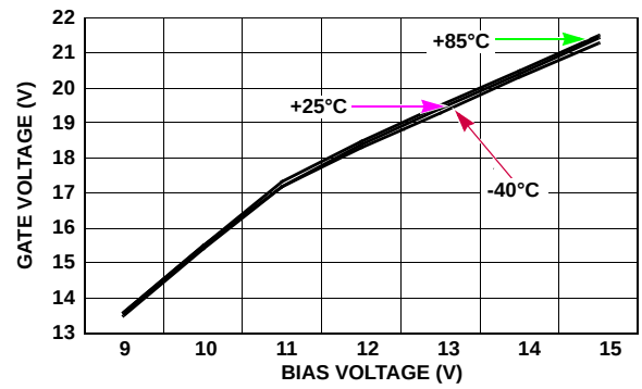
FIGURE 9. GATE VOLTAGE vs BIAS and TEMPERATURE
