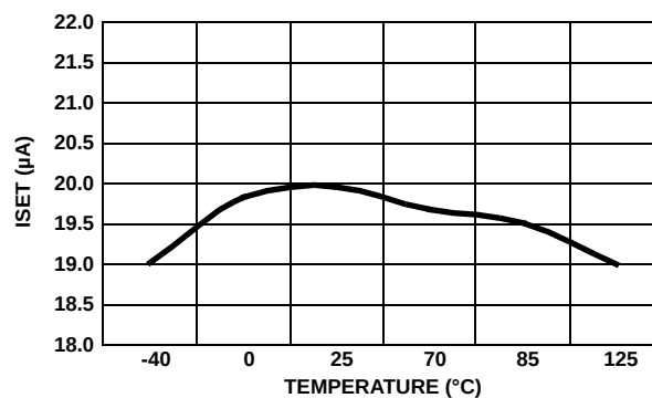
FIGURE 3. I_{SET} SOURCE CURRENT
