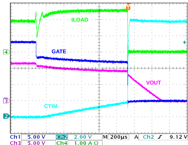
FIGURE 12. IOC REGULATION and TURN-OFF
