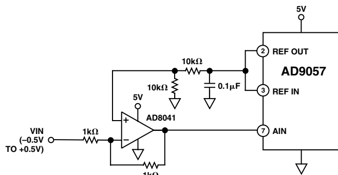
Figure 3. DC-Coupled AD9057 (Inverted VIN)
