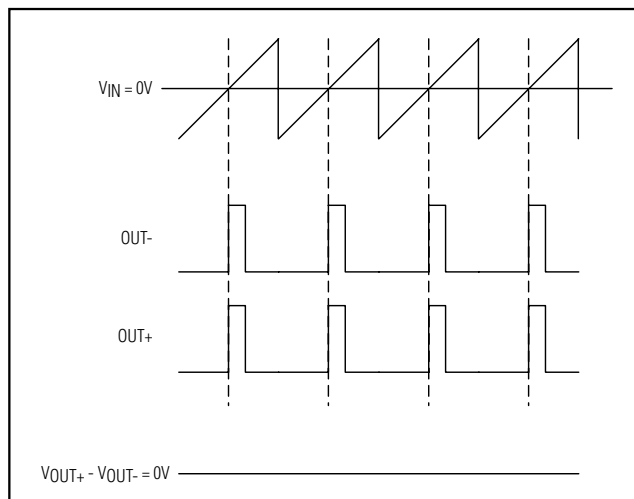
Figure 4. MAX9700 Outputs with No Input Signal
