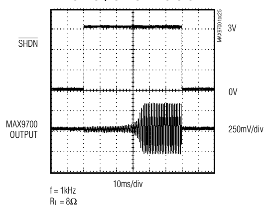
TURN-ON/TURN-OFF RESPONSE
