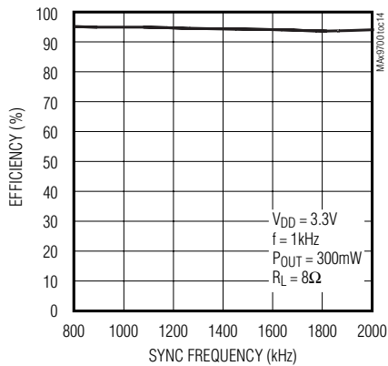
EFFICIENCY vs. SYNC INPUT FREQUENCY
