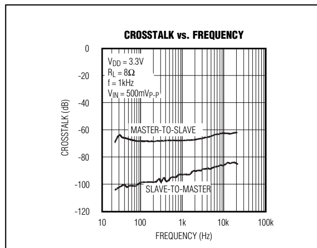
Figure 9. Master-Slave Crosstalk
