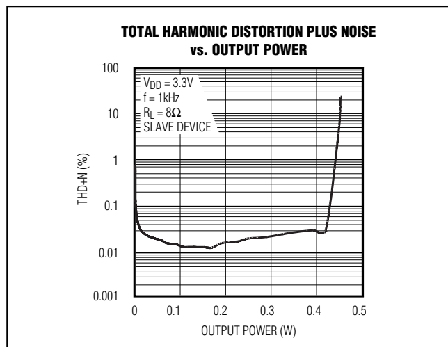
Figure 8. Master-Slave THD+N
