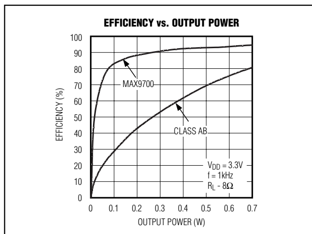
Figure 5. MAX9700 Efficiency vs. Class AB Efficiency
