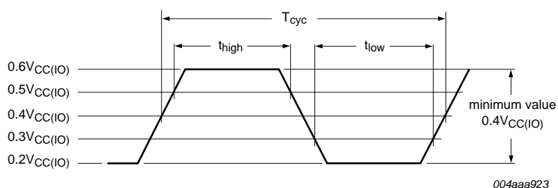
Fig 10. PCI clock
