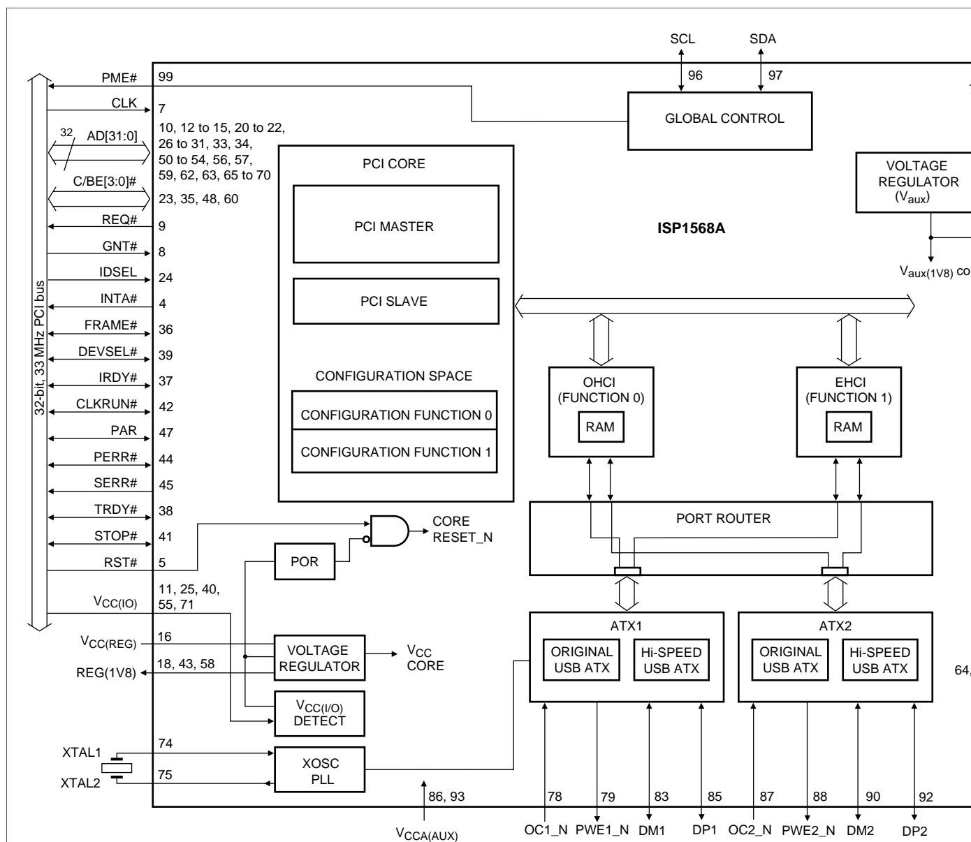
Fig 1. Block diagram
