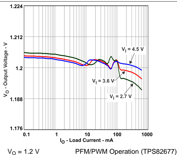
Figure 19. DC Output Voltage vs. Load Current
