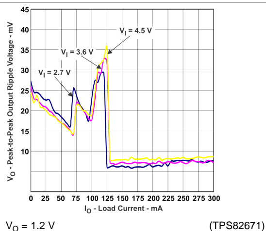
Figure 16. Peak-to-Peak Output Ripple Voltage vs. Load Current
