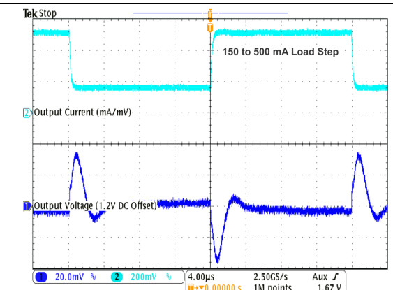
Figure 32. Load Transient Response in PFM/PWM Operation
