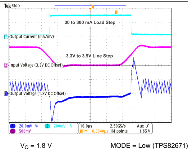
Figure 20. Combined Line/Load Transient Response
