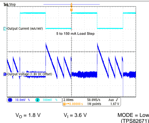
Figure 22. Load Transient Response in PFM/PWM Operation
