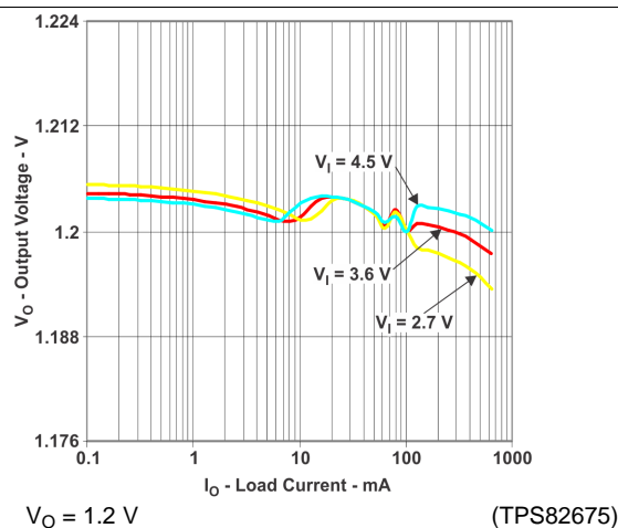
Figure 18. DC Output Voltage vs. Load Current
