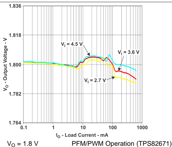
Figure 17. DC Output Voltage vs. Load Current
