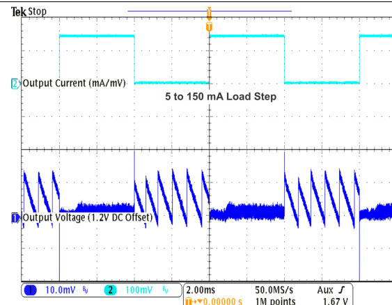
Figure 30. Load Transient Response in PFM/PWM Operation
