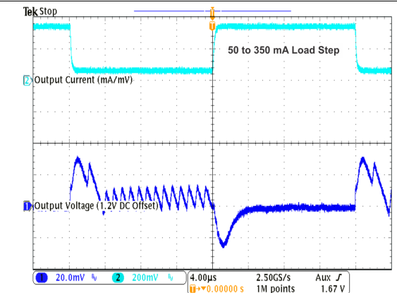
Figure 30. Load Transient Response in PFM/PWM Operation
