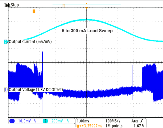
Figure 29. AC Load Transient Response
