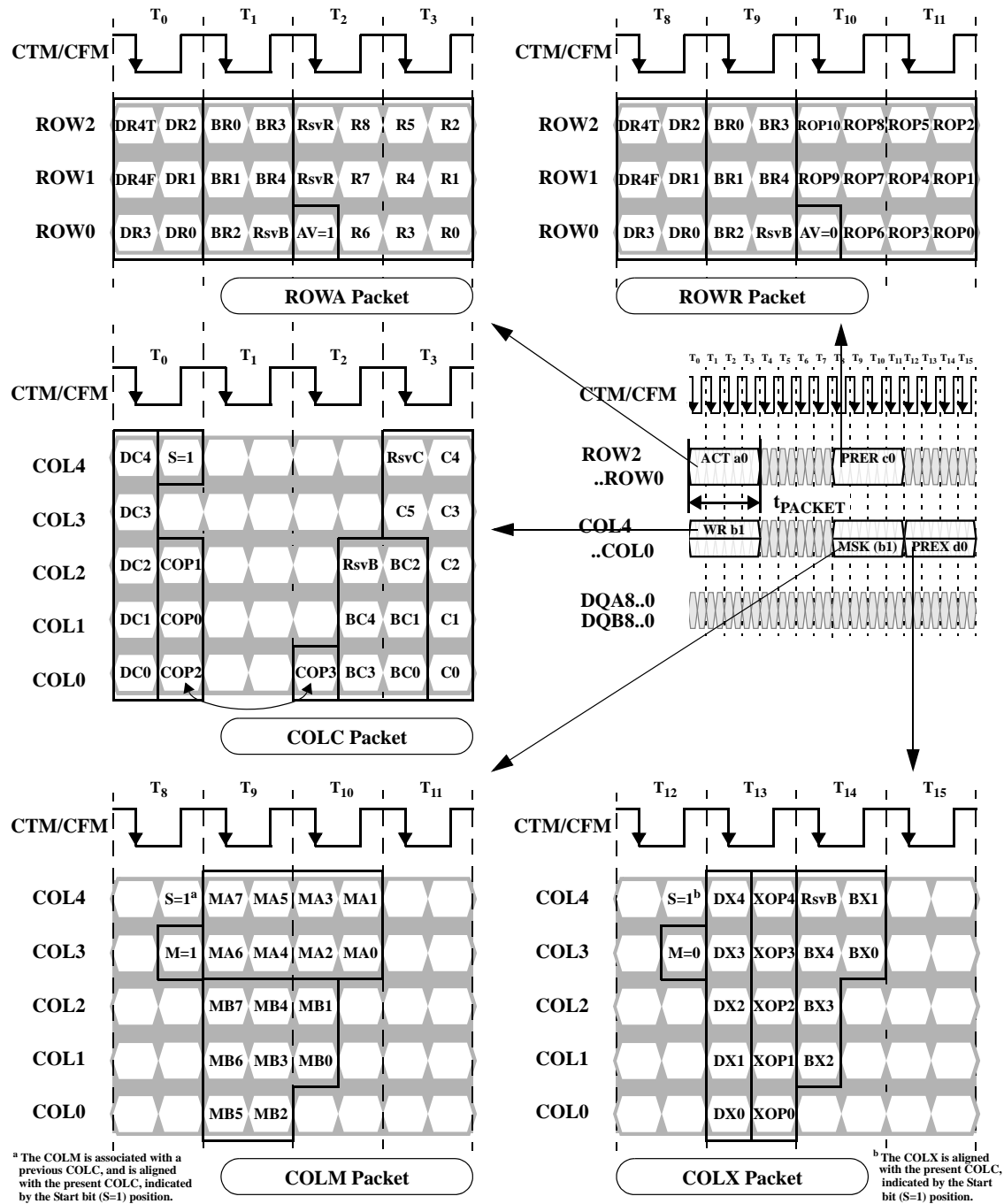
Figure 3: Packet Formats
