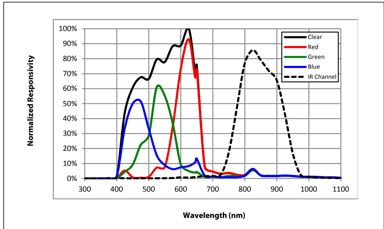
Figure 14: Spectral Responsivity
