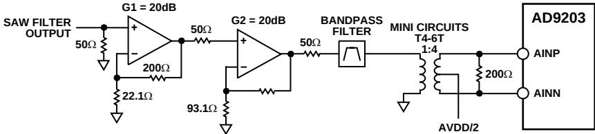
Figure 33. Simplified IF Sampling Circuit
