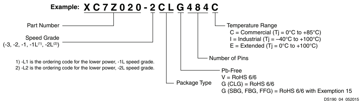
Figure 4: Ordering Information
