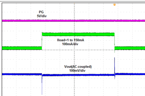
Figure 12. Load Transient Response, 10 ms/div
