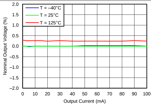
Figure 5. Load Regulation ( V_{in} = 14\text{ V} )
