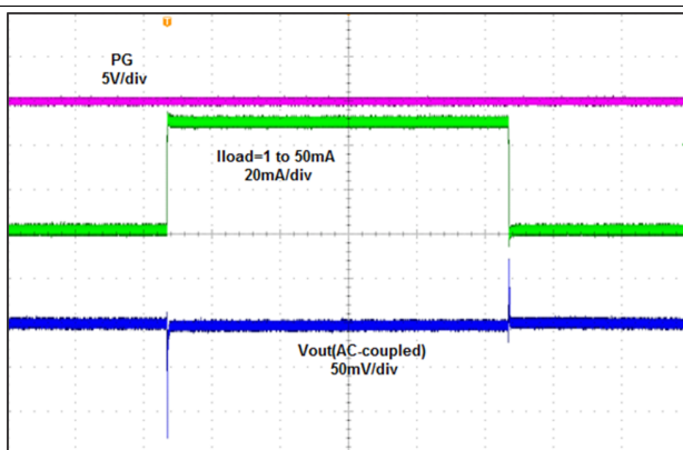
Figure 11. Load Transient Response, 10 ms/div
