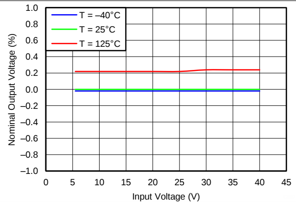
Figure 2. Line Regulation ( V_{in} = 14\text{ V} , I_L = 1\text{ mA} )
