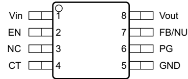
8-Pin MSOP (TPS7A66xx-Q1) DGN Package (Top View)
