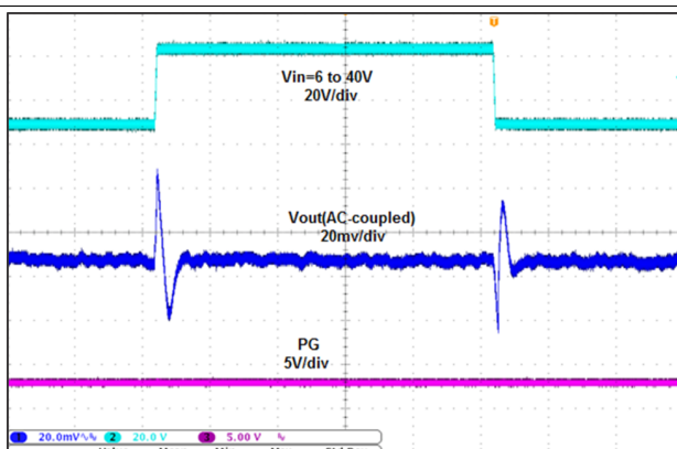
Figure 13. Line Transient Response, I_L = 1 \text{ mA} , 1 \text{ V}/\mu\text{s}
