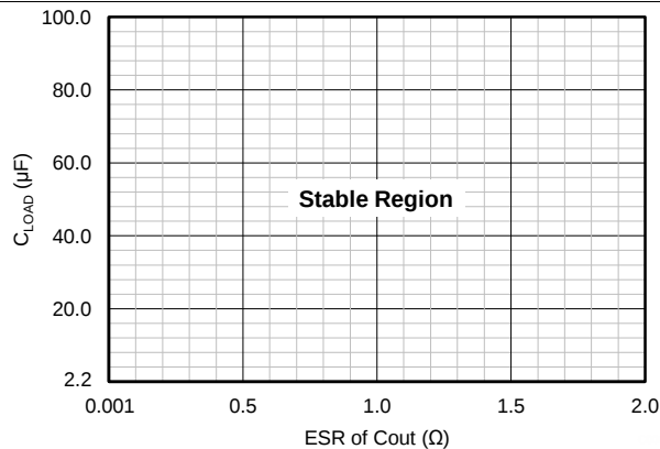
Figure 9. Load Capacitance vs ESR Stability
