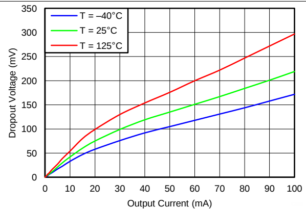
Figure 6. Dropout Voltage vs Output Current ( V_{in} = 4\text{ V} )
