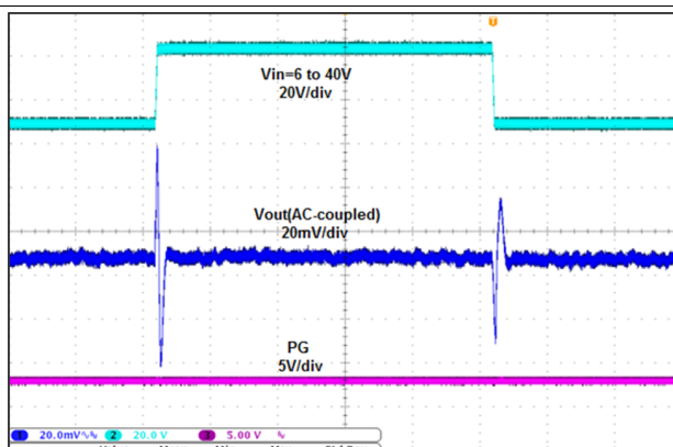
Figure 14. Line Transient Response, I_L = 10 \text{ mA} , 1 \text{ V}/\mu\text{s}
