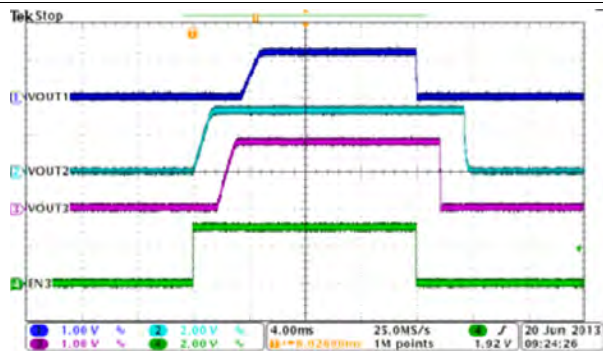
Figure 60. Automatic Power Sequencing, MODE=EN1=EN2=HIGH
