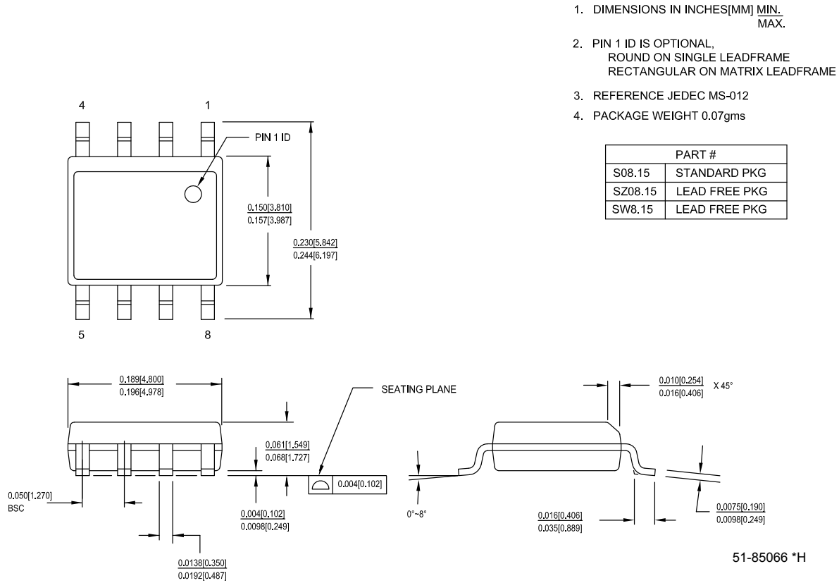
Figure 15. 8-pin (150-mil) SOIC Package Outline
