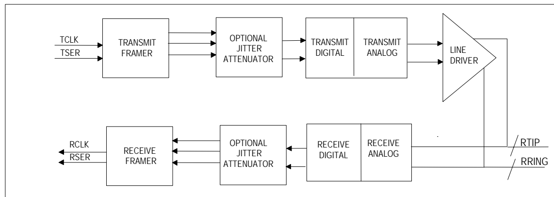
Figure 8-16. Analog Loopback
