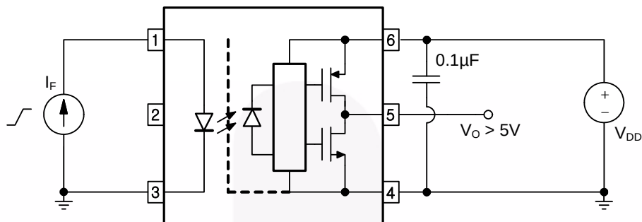
Figure 27. I_{FLH} Test Circuit
