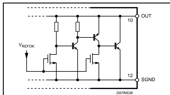
Figure 28. Pull-Down of the output in UVLO.
