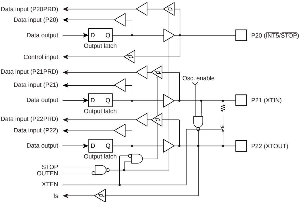
Figure 7-4 Port 2
