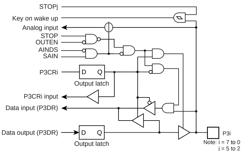
Figure 7-5 Port P3
