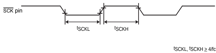
Figure 10-3 External Clock
