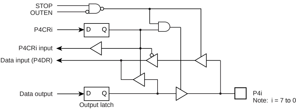
Figure 7-6 Port P4
