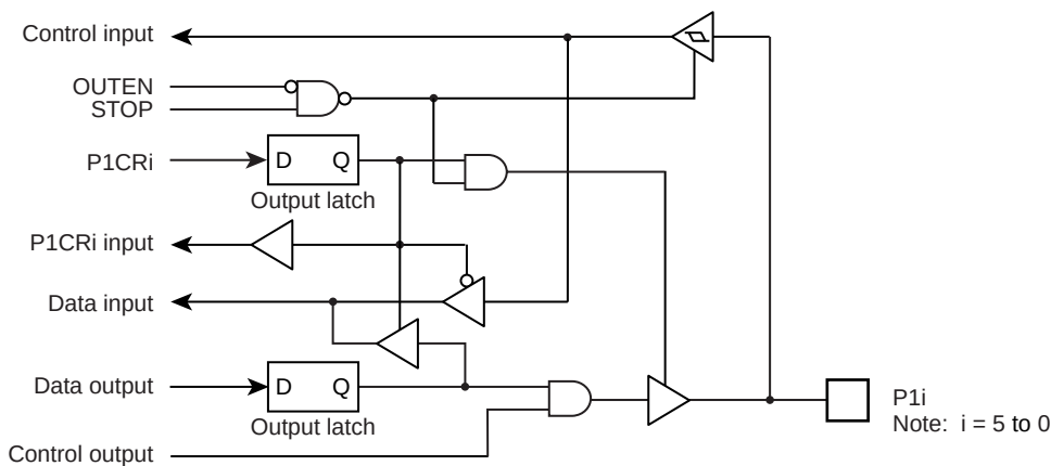
Figure 7-3 Port P1
