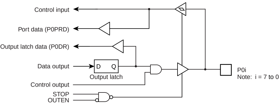
Figure 7-2 Port 0
