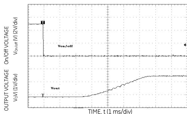
Figure 15. Typical Start-Up Using Remote On/Off with Low-ESR external capacitors (7x150uF Polymer)
