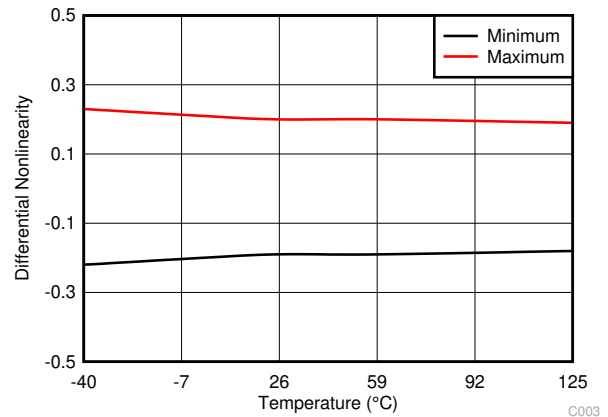
Figure 7-3. Typical DNL
