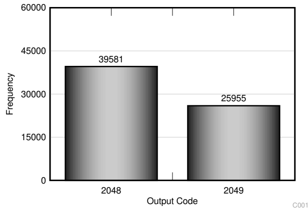
Figure 7-2. DC Input Histogram
