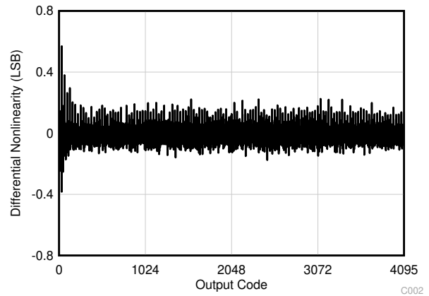
Figure 7-3. Typical DNL
