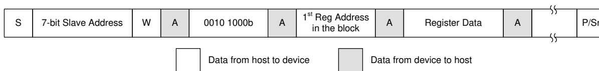
Figure 8-20. Writing a Continuous Block of Registers
