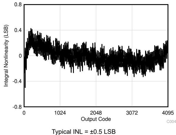
Figure 7-4. Typical INL
