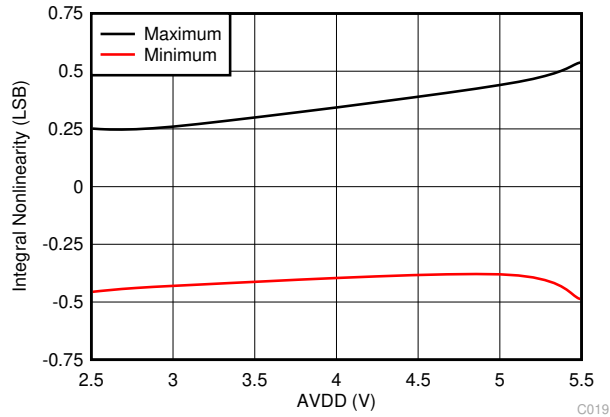
Figure 7-8. INL vs AVDD
