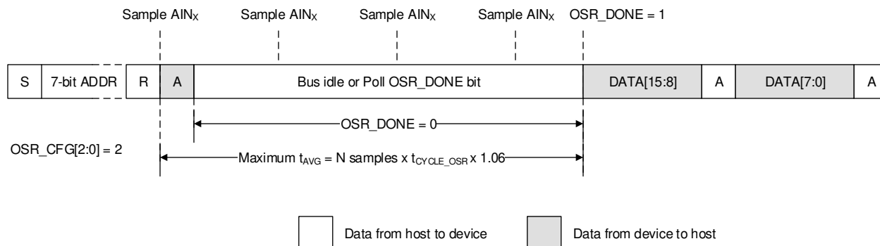
Figure 8-4. Averaging Example
