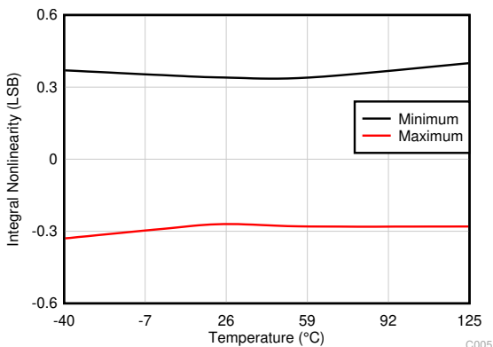
Figure 7-4. Typical INL
