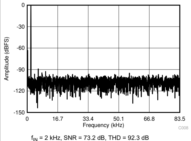
Figure 7-13. Typical FFT
