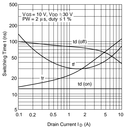
Switching Characteristics
