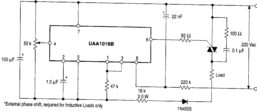
Figure 8. Electronic Rheostat
