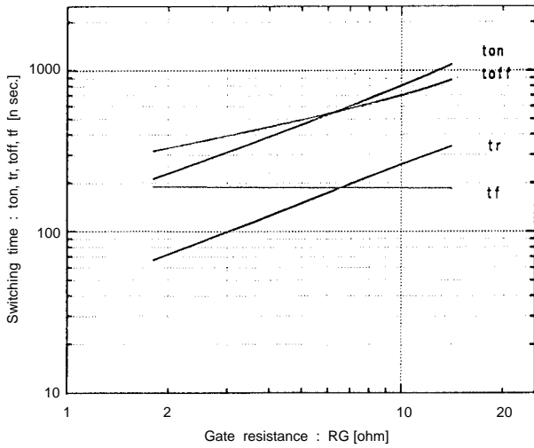
Switching time vs. RG Vcc=300V, Ic=300A, VGE=±15V, Tj=25°C
