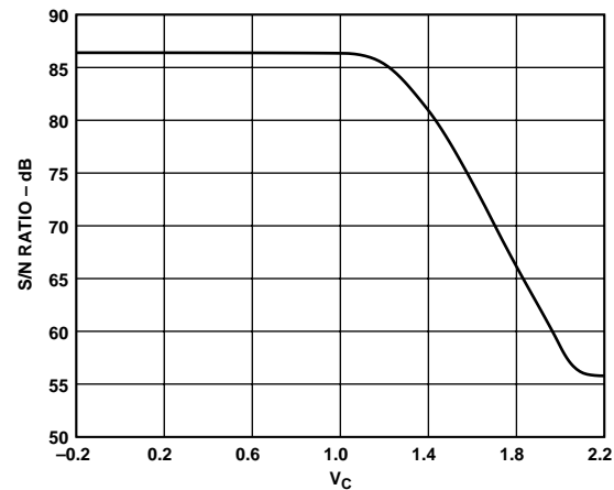
Figure 5. SNR vs. Control Voltage—Sequential Control (1 MHz Bandwidth)
